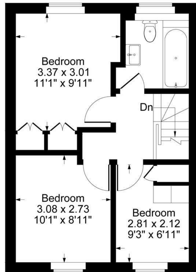
First Floor
